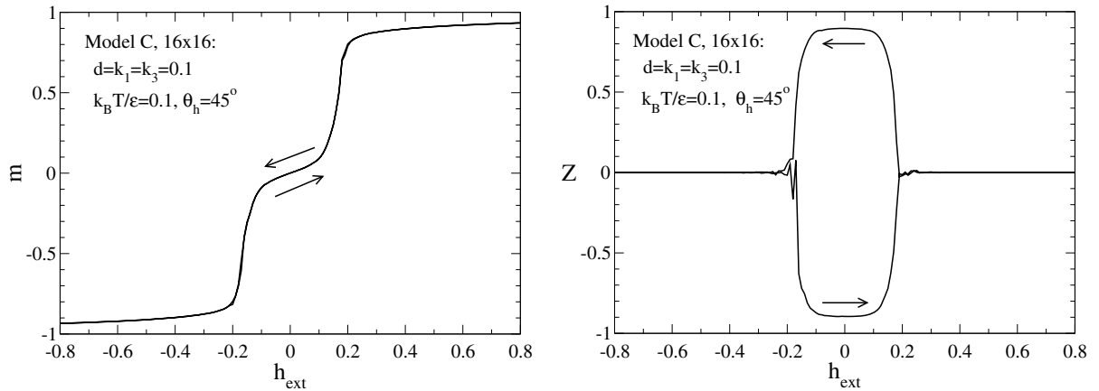
Figure 7. (Model C) With D = K_1 = K_3 = \frac{1}{10}\epsilon , at temperature k_B T = \frac{1}{10}\epsilon : (a) the averaged magnetization per site versus external magnetic field h_{\text{ext}} applied at 45^\circ above the x -axis; and (b) the order parameter Z versus h_{\text{ext}} . The field strength was initially set at h_{\text{ext}} = 0.8 and scanned to h_{\text{ext}} = -0.8 , and then back to the starting value as in a hysteresis loop calculation.
