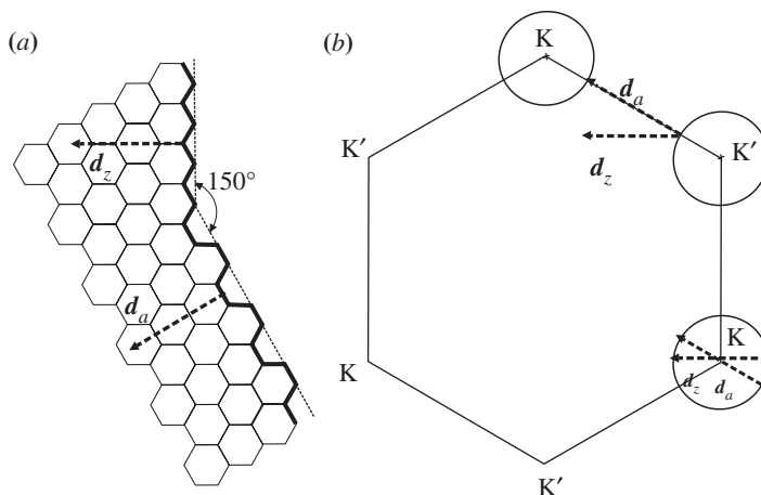
Figure 9. (a) Schematic of the atomic structure of edges in r space with the zigzag and armchair orientations. The boundaries can scatter electrons with momentum transfer along \mathbf{d}_z for the zigzag edge, and \mathbf{d}_a for the armchair edge. (b) First Brillouin zone of the two-dimensional graphite (graphene), showing defect-induced inter-valley and intra-valley scattering processes. Since \mathbf{d}_z cannot connect the K and K' points, the defect-induced double-resonance inter-valley process is forbidden at zigzag edges (Cançado et al. 2004).
