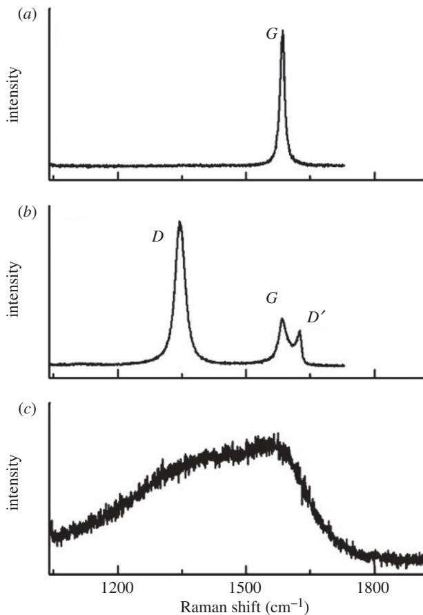
Figure 1. The first-order Raman spectrum of (a) crystalline graphene, (b) defective graphene and (c) highly disordered single-layer graphene deposited on a \text{SiO}_2 substrate. These spectra are all obtained with E_{\text{laser}} = 2.41 \text{ eV} (Jorio et al. 2010a).
