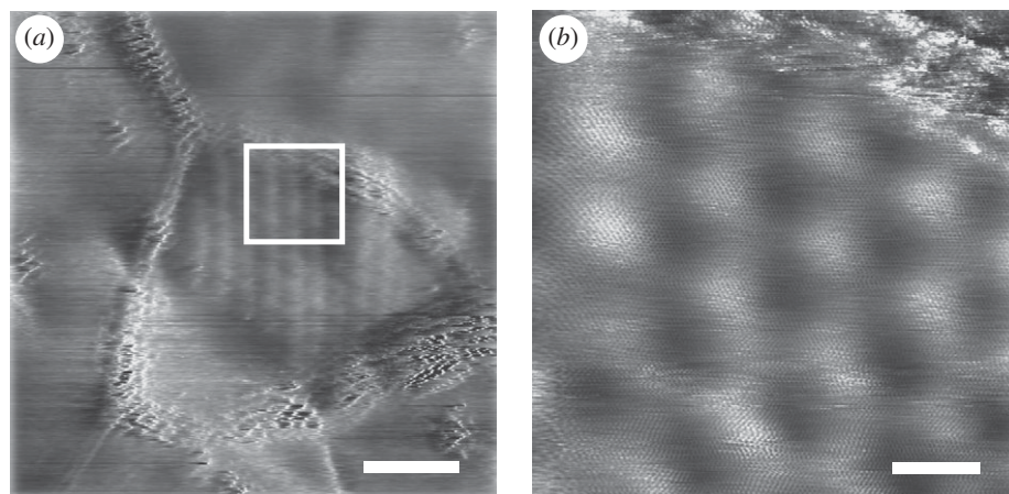
Figure 6. Scanning tunneling microscopy (STM) images with atomic resolution obtained from the surface of a nanographite crystallite of a sample with L_a = 65 nm. (a) A moiré pattern at the crystallite surface is observed (scale bar, 25 nm). (b) Magnification of the region delineated by the white square in (a), where the carbon atom positions in the graphite lattice can be more clearly observed (Cançado et al. 2007; scale bars (a,b), 5 nm).
