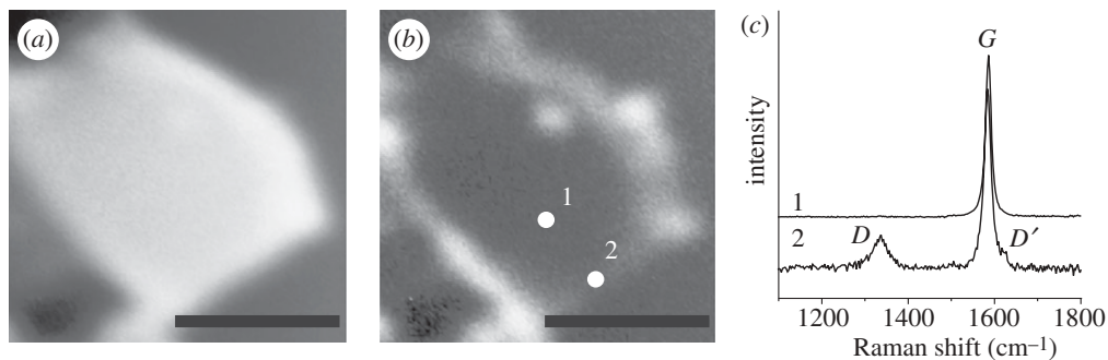
Figure 5. (a) G -band and (b) D -band confocal (300 nm resolution) Raman images of a graphite crystallite deposited on a glass substrate. In (c) the Raman spectra obtained in regions 1 and 2 (white circles depicted in (b)) are shown. The laser excitation comes from a HeNe ( \lambda = 633 nm (1.92 eV)) laser using an experimental set-up described in Pimenta et al. (2007). Scale bars, (a, b) 2 \mu m.
