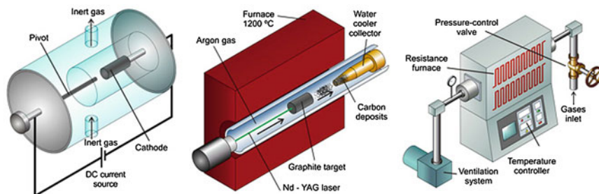
Fig. 8.2 Representative CNT synthesis methods: from left to right , electric arc discharge, laser ablation (adapted from Ref. [12]) and chemical vapor deposition
