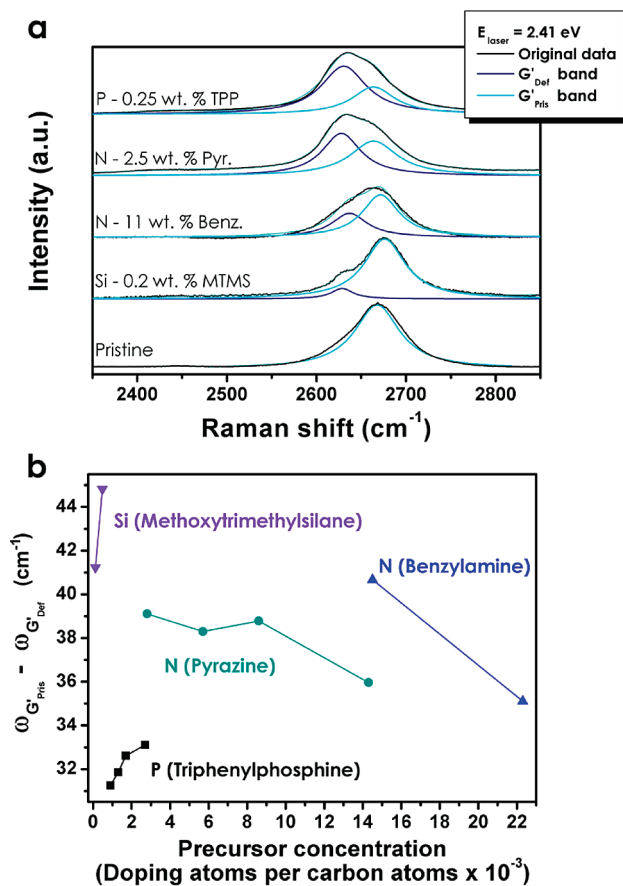
Figure 6. Raman spectra in the G' band region at E_{\text{laser}} = 2.41 \text{ eV} of the samples with maximum I_{G'_{\text{Def}}}/I_{G'_{\text{Pris}}} relative intensities for each precursor (corresponding to the highest concentrations used in this work). The blue and cyan lines correspond to the two-peak Lorentzian fitting of the G'_{\text{Def}} and G'_{\text{Pris}} bands, respectively. The spectrum of annealed pristine SWNTs at 400^\circ\text{C} is included for comparison. (b) Plot corresponding to the G' band splitting ( \omega_{G'_{\text{Pris}}} - \omega_{G'_{\text{Def}}} ) as a function of precursor concentration.
