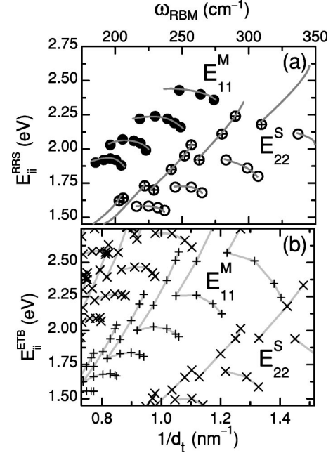
FIG. 1. (a) The electronic transition energies for SWNTs as observed by RRS ( E_{ii}^{\text{RRS}} ) vs radial breathing mode frequency ( \omega_{\text{RBM}} ). ● stand for metallic, ○ for type-I, and ⊕ for type-II semiconducting SWNTs. (b) The electronic transition energies calculated by the ETB ( E_{ii}^{\text{ETB}} ) from Ref. 27 (crosses for semiconducting and pluses for metallic SWNTs) vs 1/d_t . The gray lines connect SWNTs belonging to the same (2n+m) = \text{const} family.
