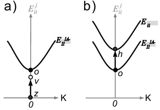
FIG. 5. Schematic diagram of two possible scenarios for the photoinduced absorption process when E_{\text{probe}} does not correspond to excitonic band-edge energies. (a) A band-edge exciton at o is created by exciting an electron from ground state z to virtual state v and combining with an optical phonon. (b) A band-edge exciton at o can combine with a photon and access a higher continuum mobile band state at E_{ii} , denoted by h .
